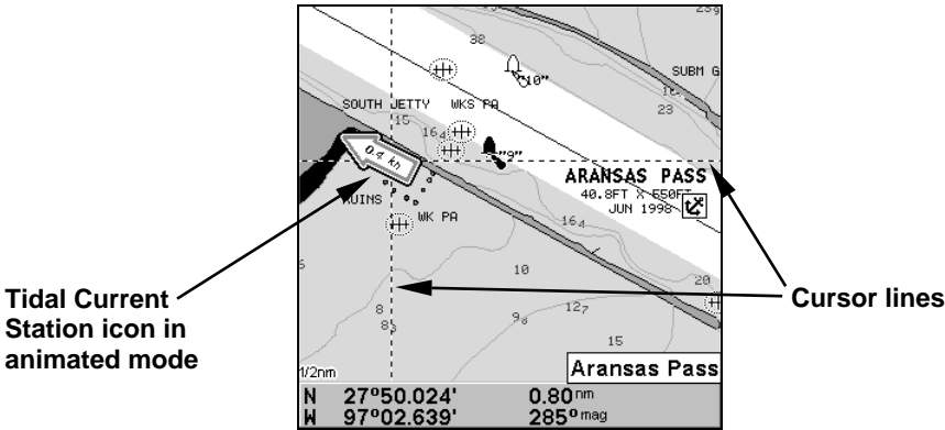
Navionics chart showing Tidal Current Station icon selected by cursor. The icon animates automatically without selecting it at the 1/2 mile zoom range. The tidal current is flowing toward the northwest at a velocity of 0.4 kn.
